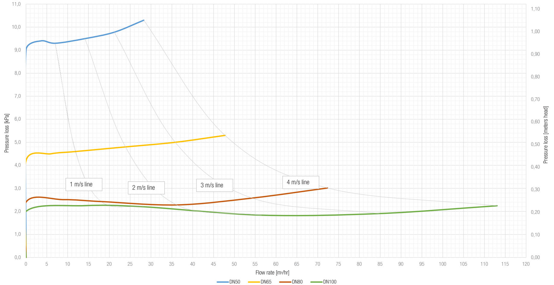
Pressure loss - series 41 - weight positioned for fastest closing - DN50, DN65, DN80 and DN100
